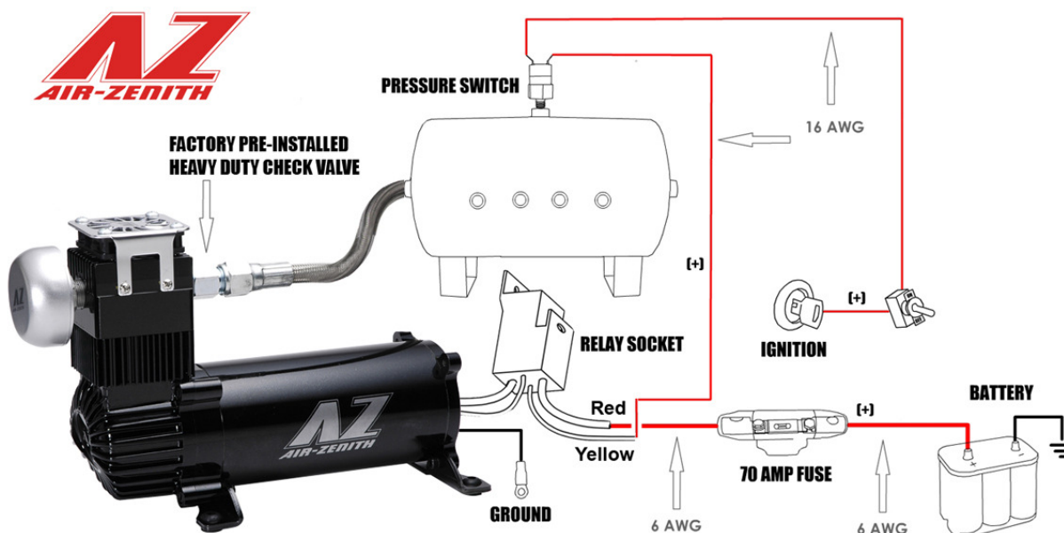
(Fig. 1 Standard Wiring Diagram)
